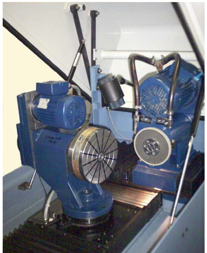
Flexible circular knife support with encoder
